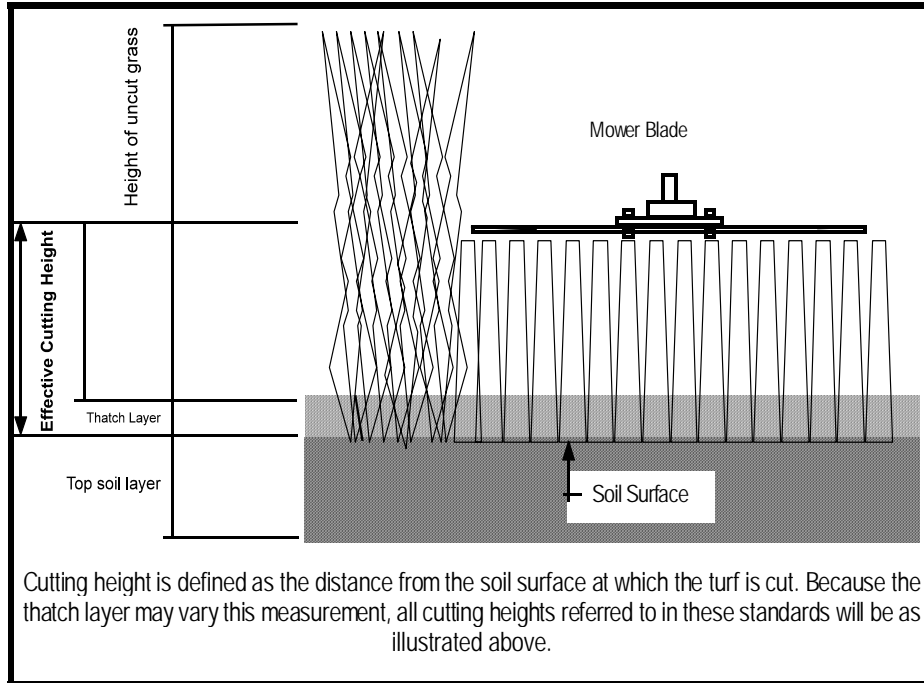
Diagram illustrating the effective cutting height
